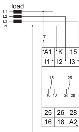
G2JM5AL20 with power modul 230V AC with fault latch
