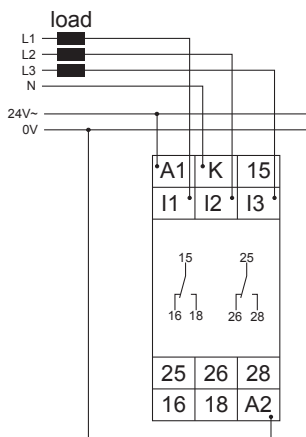
G2JM5AL20 with power modul 24V AC without fault latch
