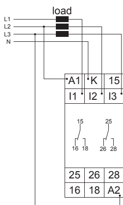
G2JM5AL20 with power modul 400V AC without fault latch
