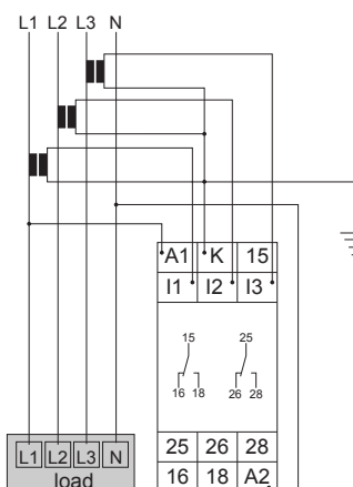
G2JM5AL20 with power modul 230V AC and current transformer
